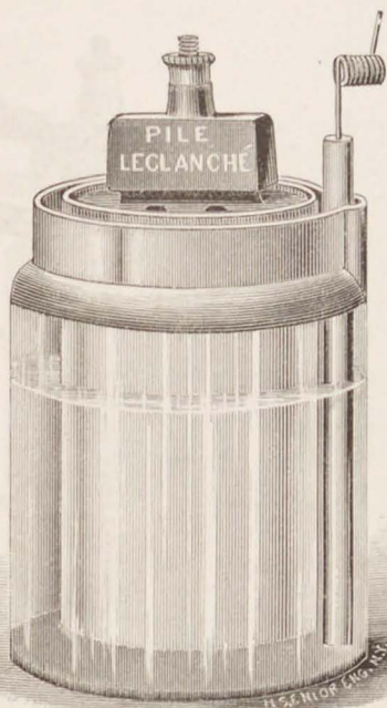
"Disque Battery," complete.
