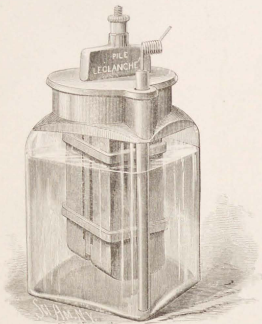
"Prism Battery" Complete.
