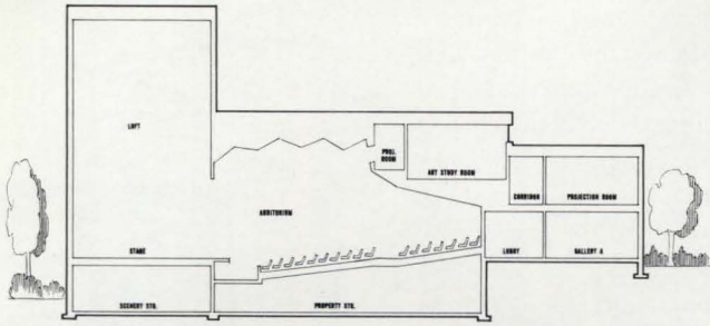
Section Drawing of Fine Arts Center
